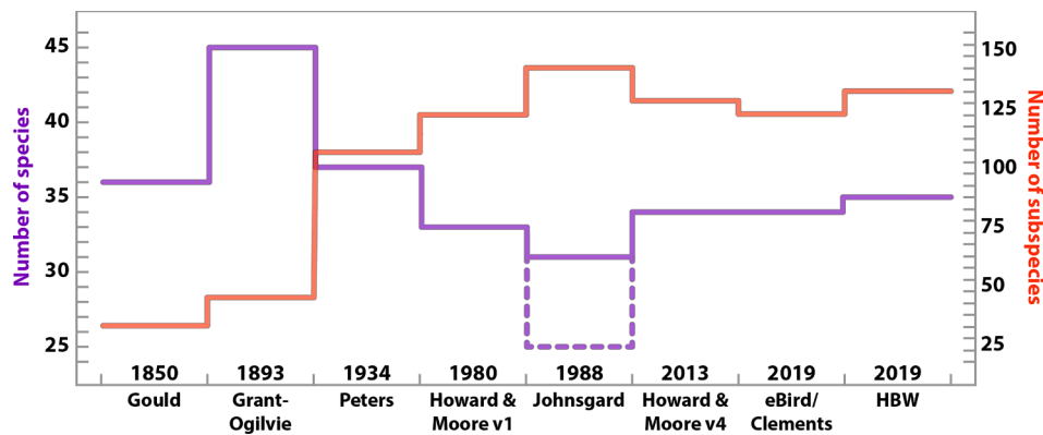
Fig. 2. Changes in odontophorid taxonomy through time with different classification schemes (x-axis). The number of species (purple) is shown on the left axis; the number of subspecies (red) is shown on the right axis. Publication year is listed above the x-axis. Dotted line at Johnsgard (1988) shows the number of species when closely related allopatric species are collapsed to subspecies. HBW = Handbook of the Birds of the World Alive.
