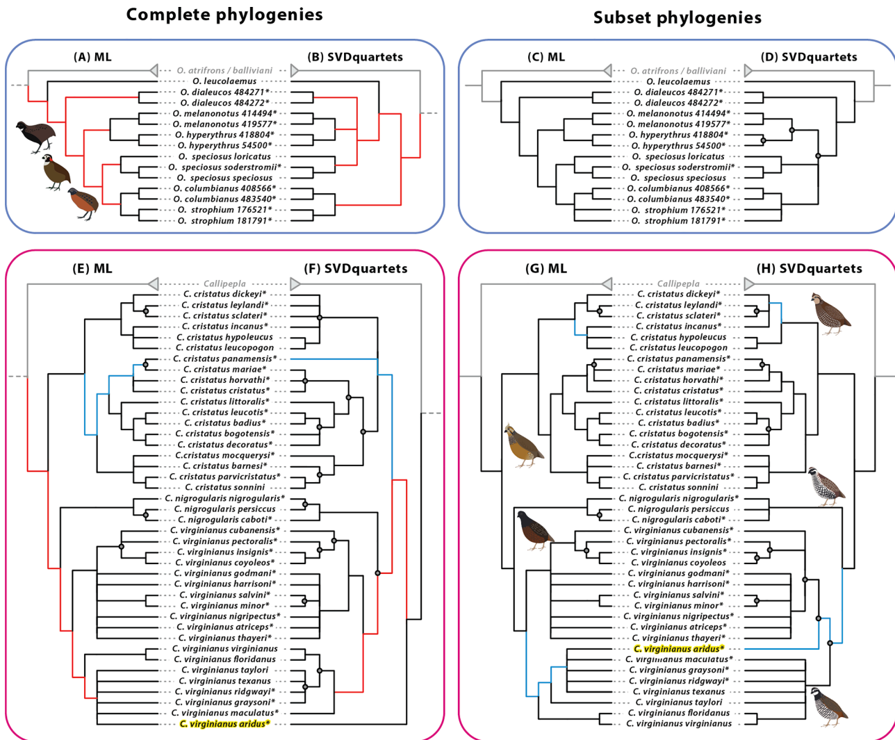
Fig. 4. Cladogram of discordant subspecies-level relationships inferred with maximum likelihood (ML) analysis and SVDquartets analysis of 3,884 nuclear ultra-conserved element loci within (A–D) Odontophorus and (E–H) Colinus . Left panels (A, B, E, F) zoom in on the relationships inferred for these clades in analyses of the complete 131 taxon dataset (Fig. 3, Supplementary Fig. S3); right panels (C, D, G, H) show relationships inferred using only the subset of taxa depicted. Asterisks denote data collected from historical museum specimens. Nodes with > 95% bootstrap support are unlabeled; gray circles = 70–94% bootstrap support; nodes with < 70% bootstrap support have been collapsed to polytomies. Red branches indicate conflicting species relationships; blue branches indicate conflicting subspecies relationships. Note position change of C. virginianus aridus (highlighted in yellow) between complete and subset phylogenies. For branch lengths and the uncollapsed ML tree of all taxa, see Supplementary Fig. S1; for the uncollapsed SVDquartets tree of all taxa, see Supplementary Fig. S2.
